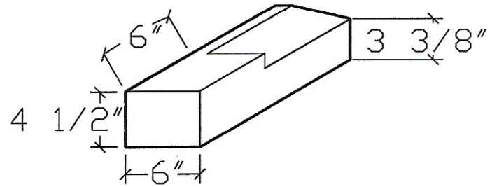
SI-B (DROPLIP SILL)
